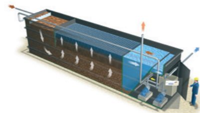
Split-O-Mat® BSB
